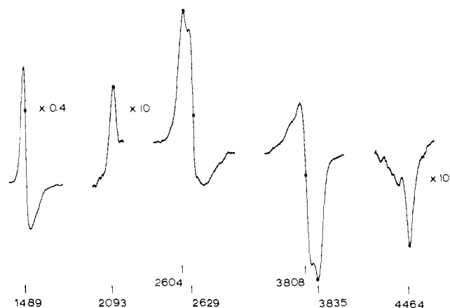
Figure 1. Epr spectrum of 9,9'-dianthrylmethylene in 9,9'-dianthryl ketone at 140°K with h\nu/g\beta = 3273.5 G.
